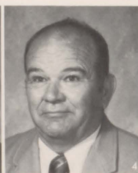
Resource Math
